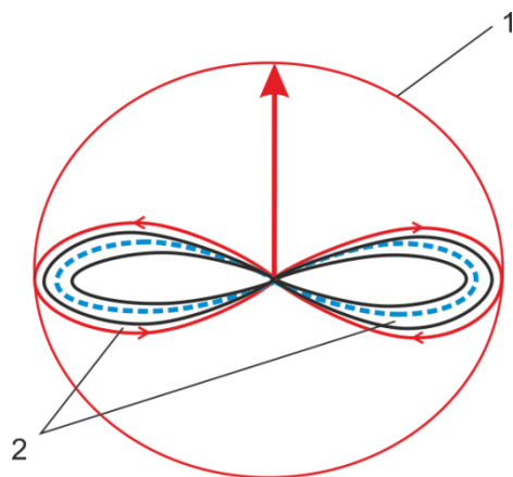
Fig. 4. Schematic Illustration of the Universe.
