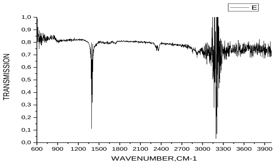
Fig. 3 Spectral Illustration of the Unified "Superperfect Energy"
