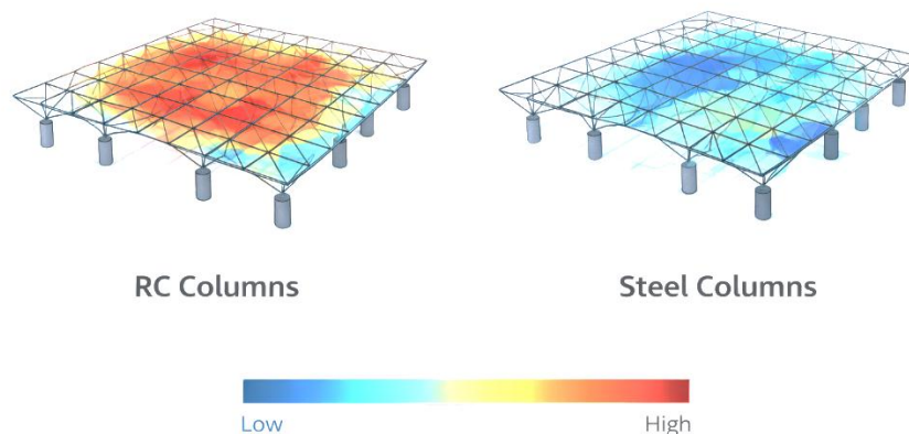
Figure 5. Comparative axial force density maps for reinforced-concrete and steel-supported space-frame roofs
