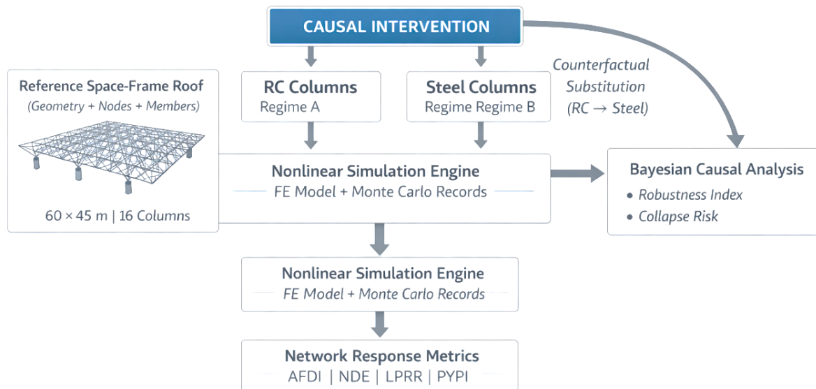
Figure 1. Methodological workflow for causal-topological seismic analysis of space-frame roof systems
